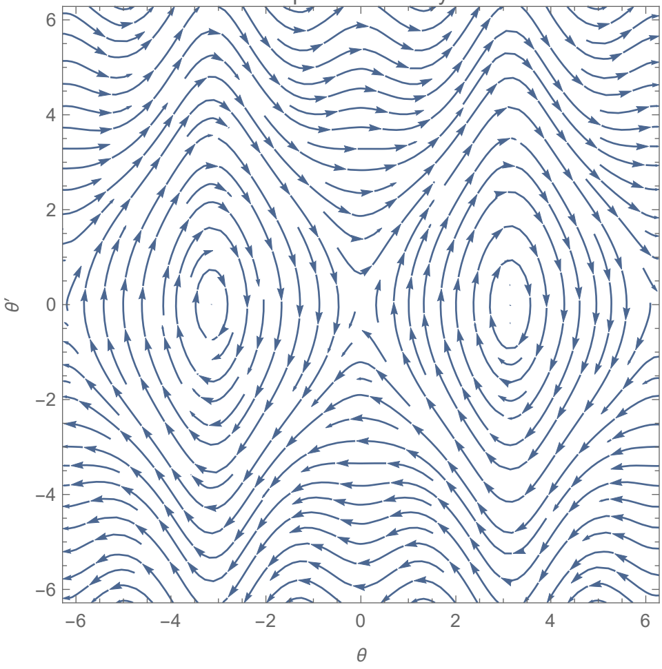
Phase portrait of the system
