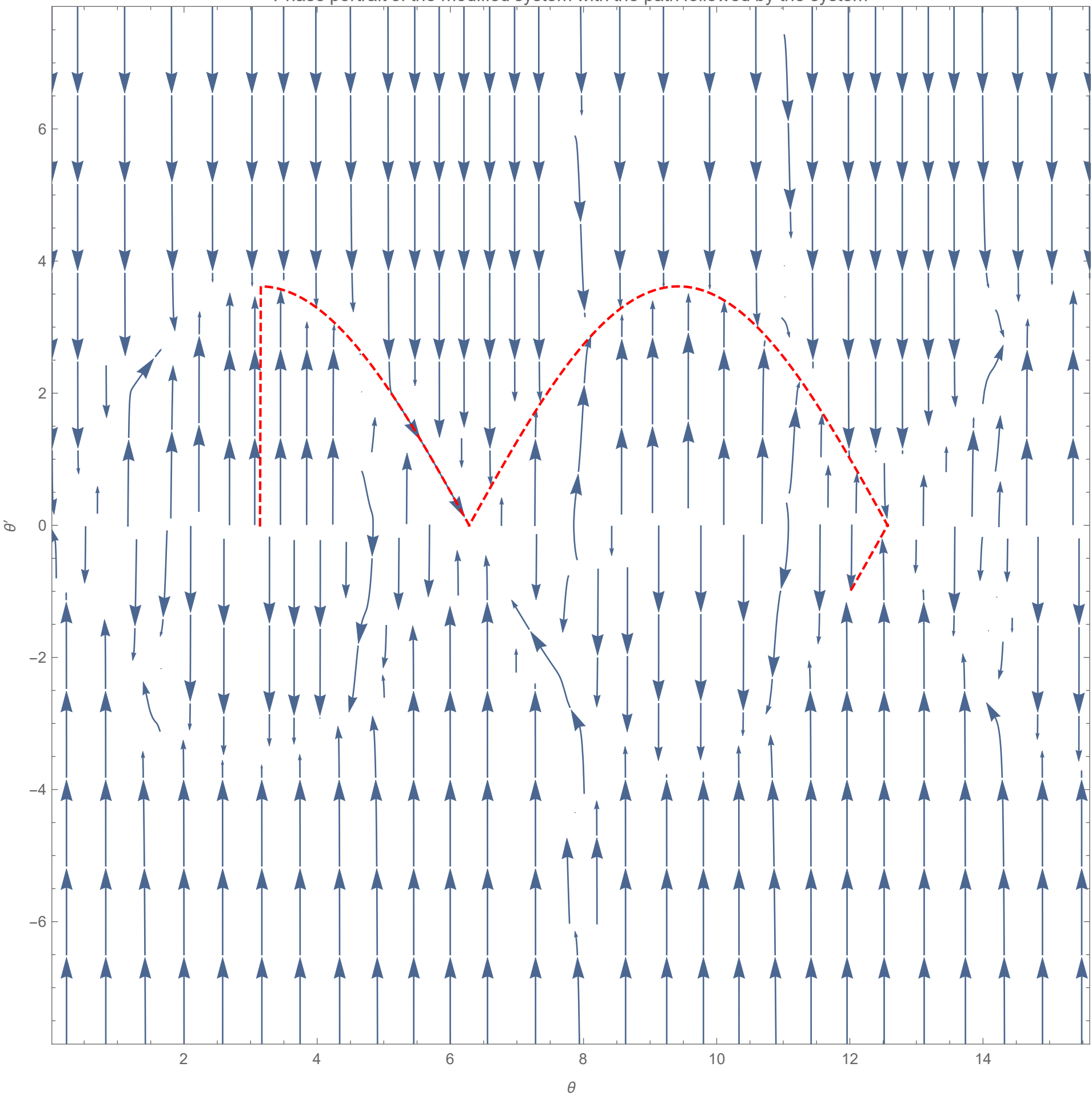
Phase portrait of the modified system with the path followed by the system
